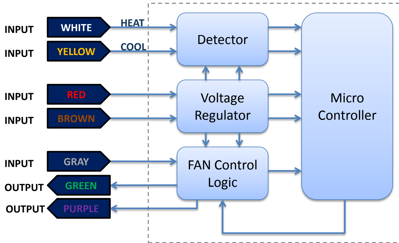
Block Diagram
